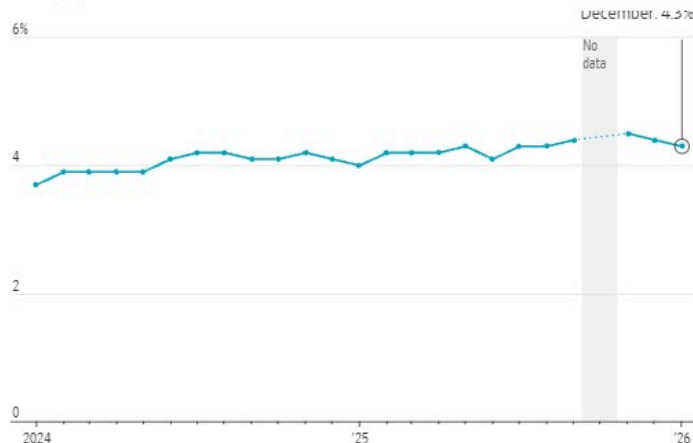
Unemployment rate
